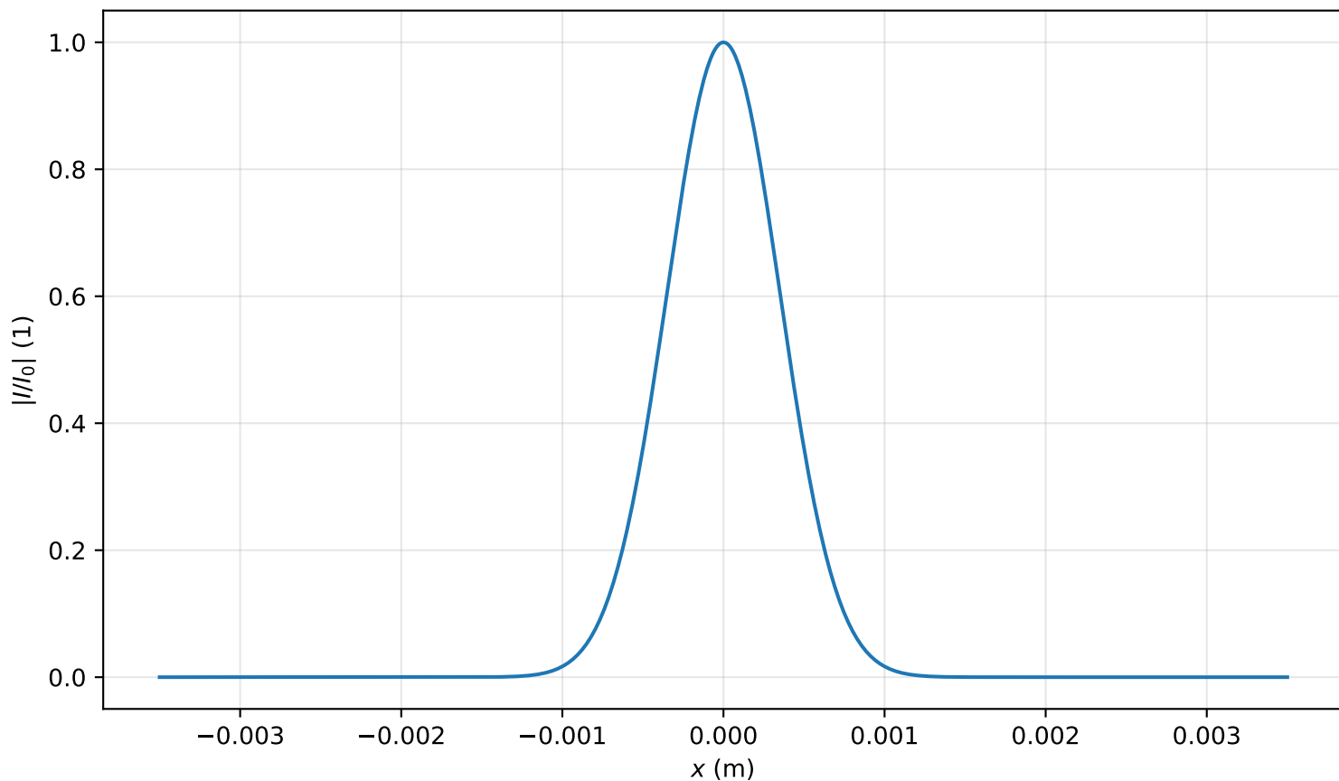
Intensity profile I(x, y = 0, z = 0.000m)/I_0 , P_{in}=0.4P_{cr} , artificial time
